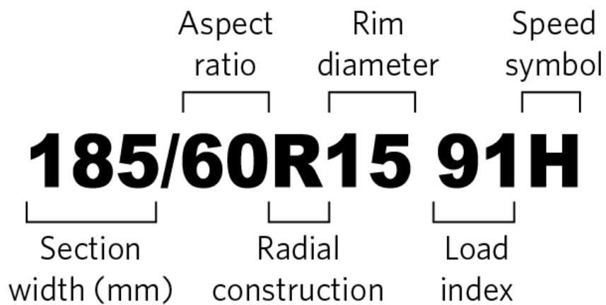
Figure 10-1-2. Tyre markings
